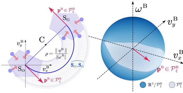
Fig. 4: Arc transitions ( Left ) and the set of allowed velocities \mathcal{P}_\xi^B ( Right ) visualized on a unit sphere.
