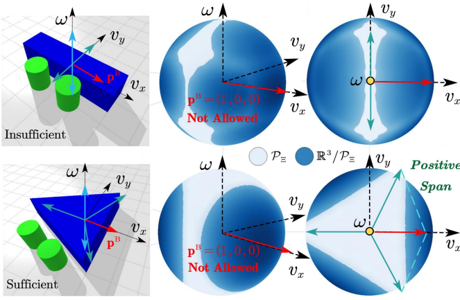
Fig. 6: Given all modes \Xi for two robots and different objects (Left), the set of allowed velocities \mathcal{P}_\Xi is shown (in white) on a unit sphere of v_x - v_y - \omega velocities (Middle) with the top-down projection (Right) from the angular velocity \omega .
