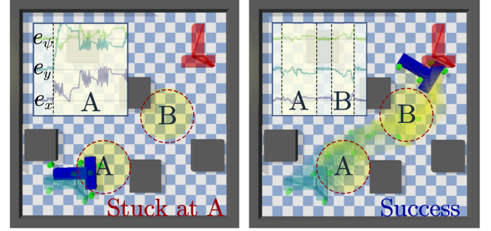
Fig. 16: Robustness to temporary “blackout” (in Regions A and B), where no measurements of the object state are obtained. Final trajectories and state estimation error are shown by linear extrapolation (Left) and constrained EKF (Right).
